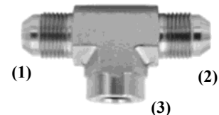
(1) JIC male, (2) JIC male, (3) NPTF female Parker OTX-S SAE# 070427 Parker 223T Aeroquip 2031 (Reversed) Weatherhead C5655
