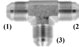
(1-3) JIC male Parker JTX-S SAE# 070401 Parker 033T Aeroquip 2033 (Reversed) Weatherhead C5705
